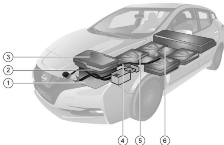
High-voltage components
